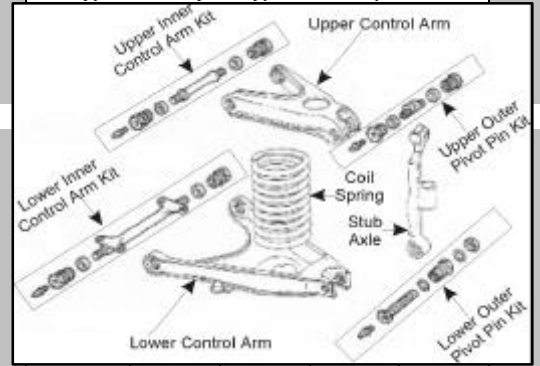
Typical of Early GM type Front Suspension
